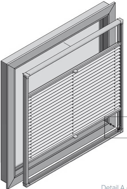
Detail A - 1
