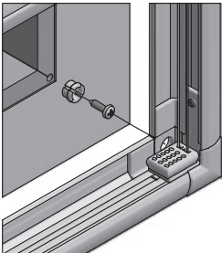
Detail A - 1
