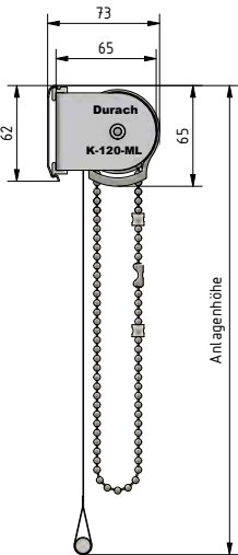
Wandmontage
