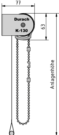
Wandmontage
