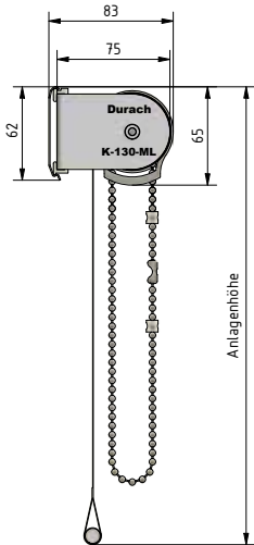
Wandmontage
