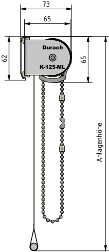
Wandmontage
