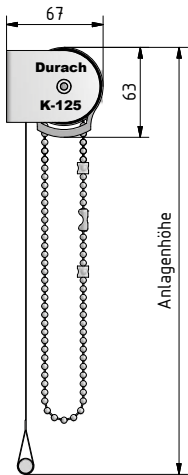
Wandmontage
