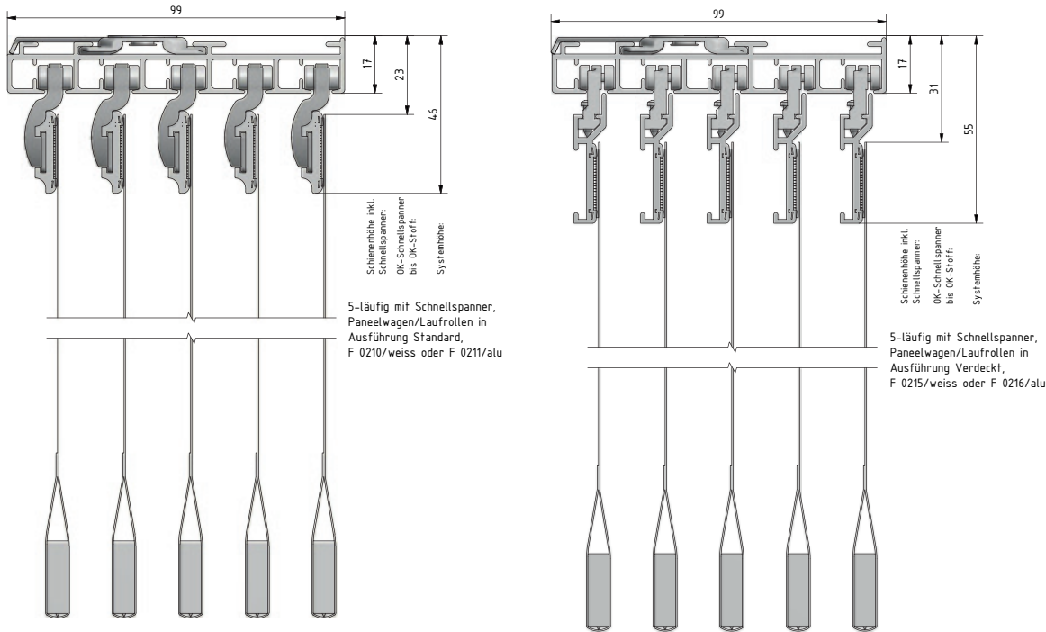
Paneelwagen Standard
