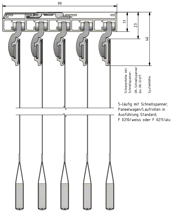
Paneelwagen Standard
