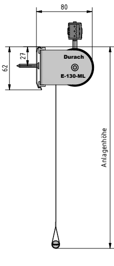
Wandmontage
