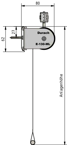
Wandmontage
