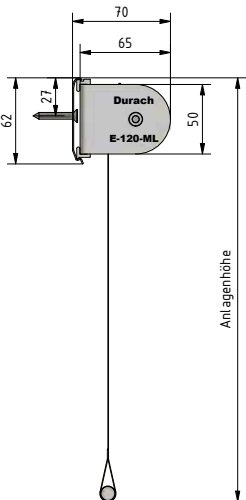
Wandmontage
